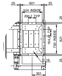
DETAIL A 1:20
